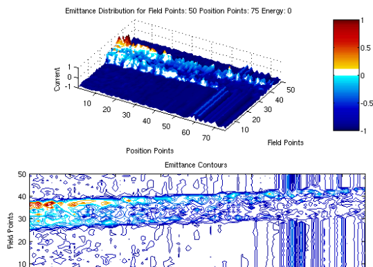
Figure 2: An example of the displayed pulsed beam emittance scan
