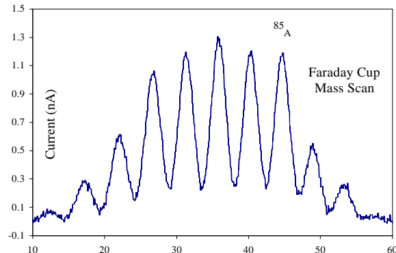
Figure 1: Mass scan
